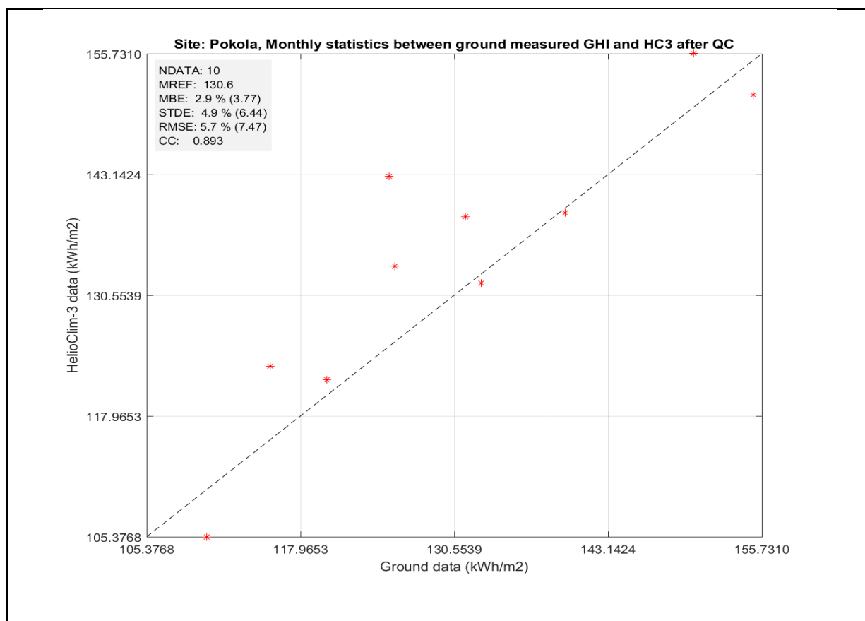
Figure 7: GHI statistical results before calibration - monthly values
