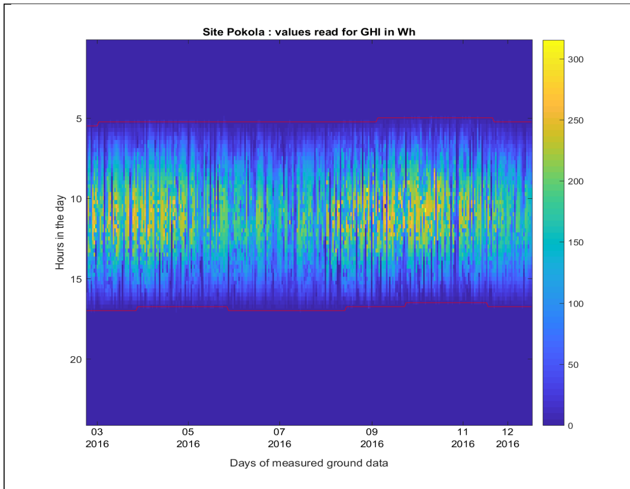
Figure 1: GHI from the ground station
