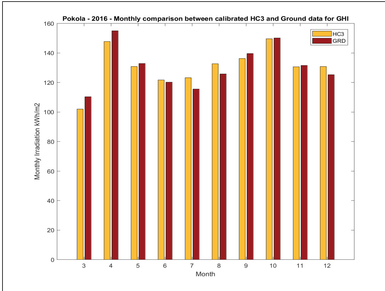
Figure 9: GHI monthly values comparison
