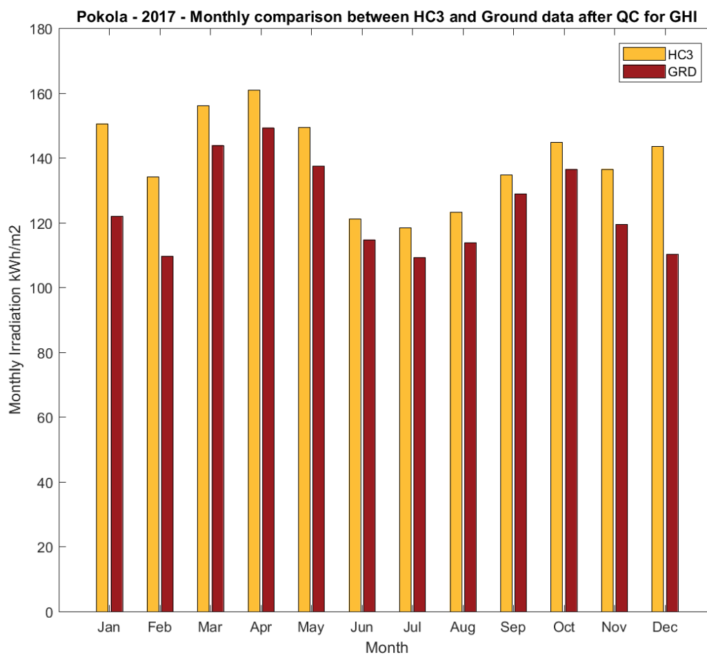
Figure 11: GHI monthly values comparison for the year 2017
