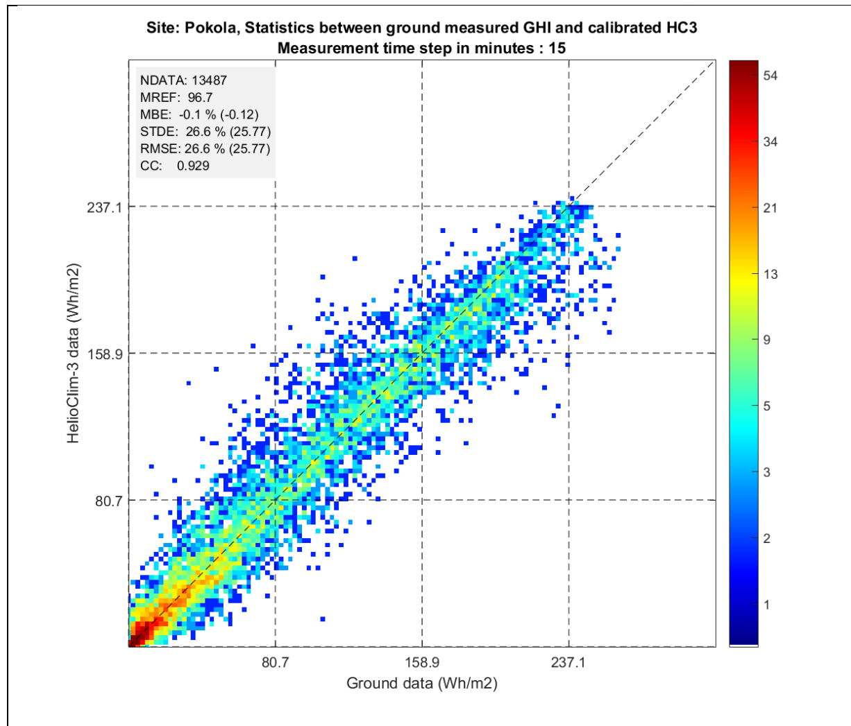
Figure 8: GHI statistical results after calibration – measurement time step values
