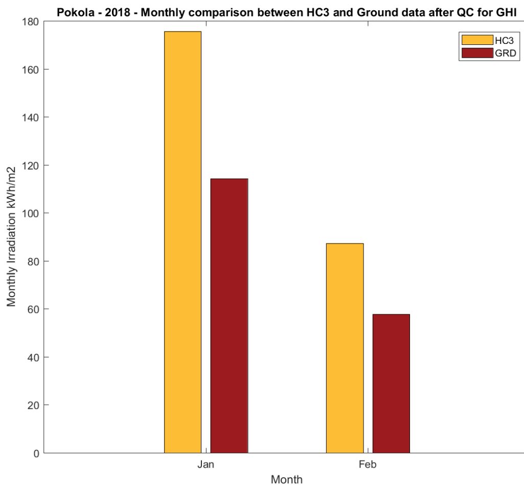
Figure 12: GHI monthly values comparison for Jan. and Feb. 2018
