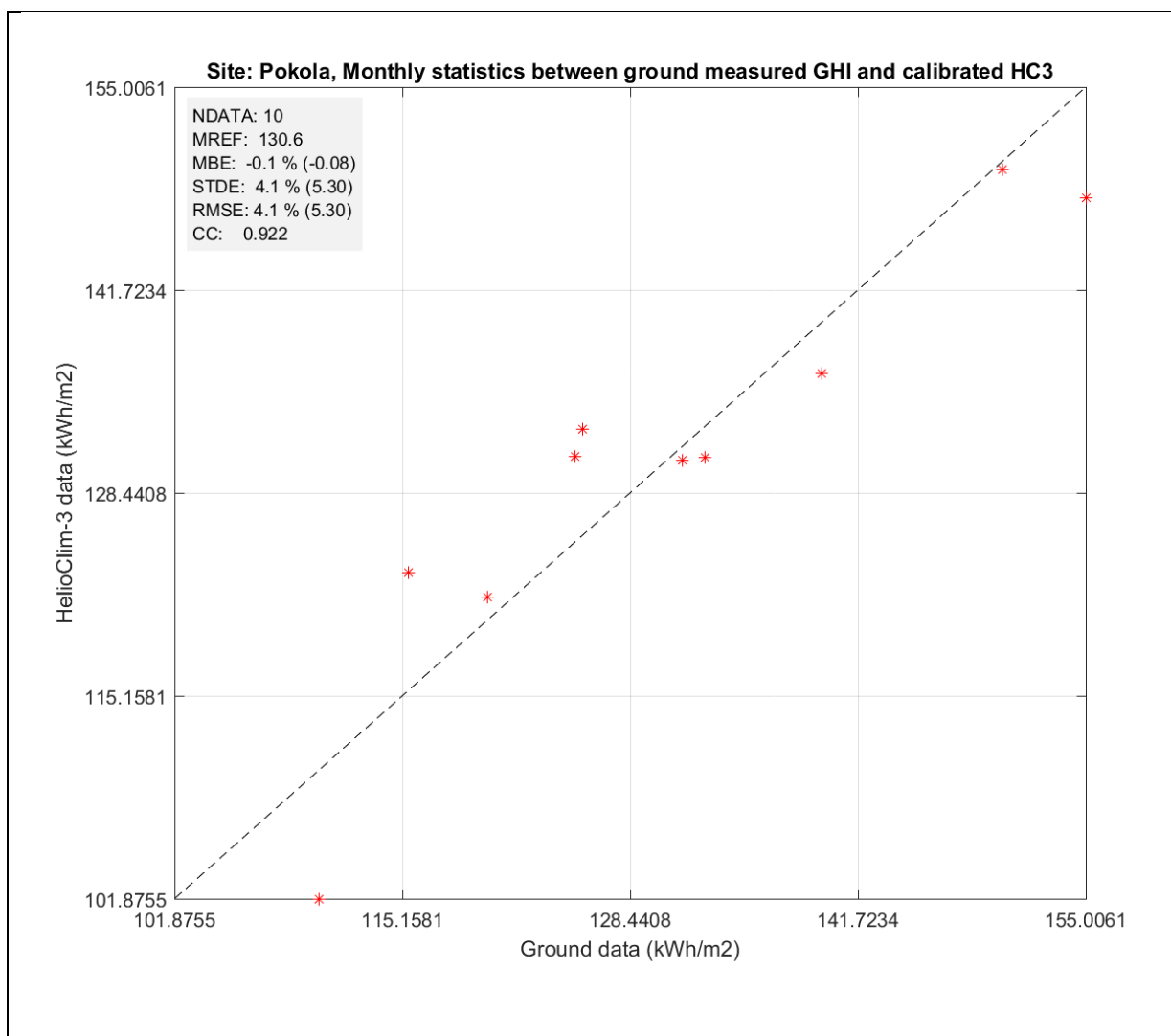
Figure 10: GHI statistical results after calibration - monthly values
