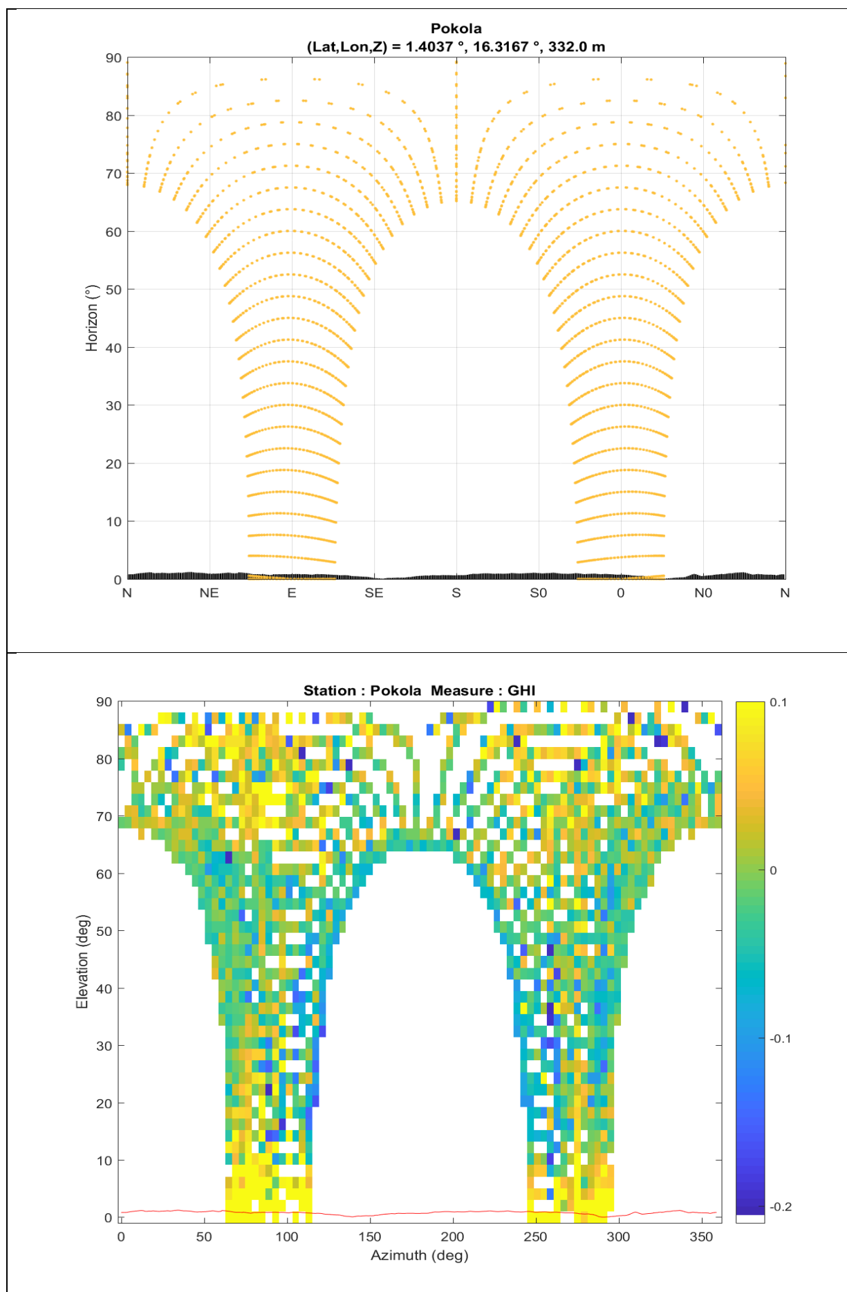
Figure 3: horizon and sun path and near shadowing
