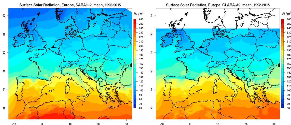
Figure 2. Mean surface solar radiation ( \text{W/m}^2 ) (1992–2015) based on the (left) SARAH-2 and (right) CLARA-A2 climate data record.
