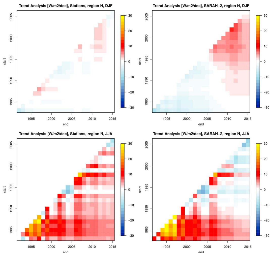
Figure 12. Trendraster-plots of mean SSR trends derived from (left) stations and (right) SARAH-2, for the (top) winter and (bottom) summer season for the region north. The y axis denotes the start years, and the x axis shows the end years of the individual trends. Trendrasters show linear trends ( \text{W/m}^2/\text{decade} ) during time periods of at least 10 years (at the diagonal); the trend over the maximum time period analyzed is shown by the pixel at the lower right end.
