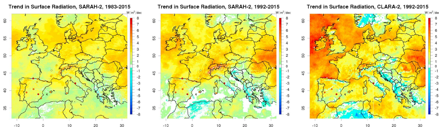
Figure 7. Spatial distribution of the linear trends ( \text{W/m}^2/\text{decade} ) of surface solar radiation during 1983–2015 for (left) SARAH-2 and during 1992–2015 for (middle) SARAH-2, and (right) CLARA-2. The respective trends for the 53 stations are shown as colored dots.
