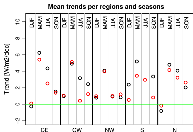
Figure 8. Trends ( \text{W/m}^2/\text{decade} ) of surface solar radiation of (black) stations and (red) SARAH-2 data, shown separately for region and season during the full time period of 1983–2015. Regions: CE = central east, CW = central west, NW = northwest, S = south, and N = north.
