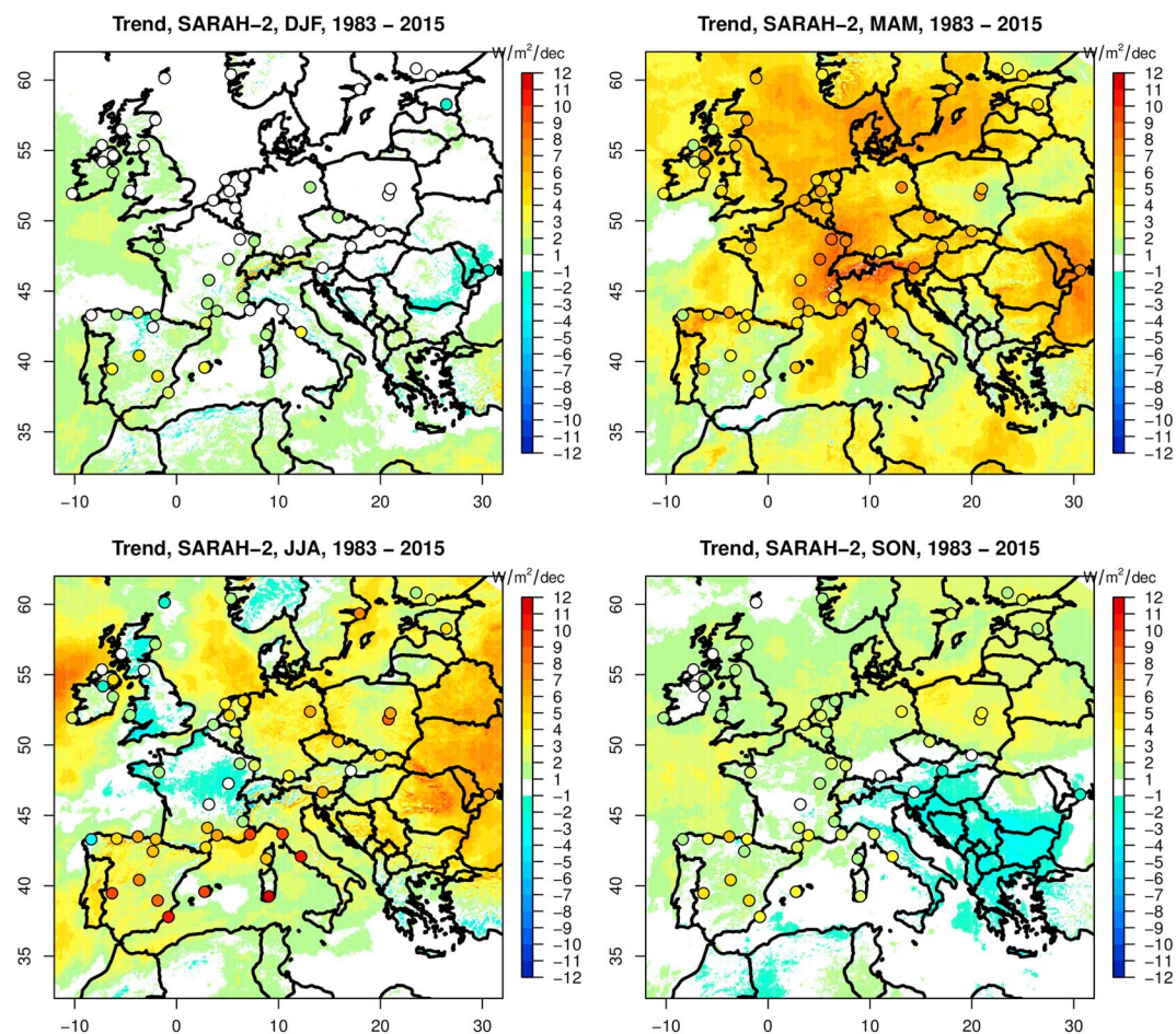
Figure 10. Spatial distribution of the linear trends ( \text{W/m}^2/\text{decade} ) of surface solar radiation during 1983–2015 for the four seasons (DJF, MAM, JJA, and SON) based on the SARAH-2 climate data record. The trends for the respective season and time period given by the 53 stations are shown as colored dots.
