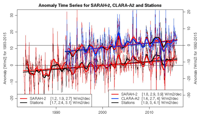
Figure 4. Mean monthly anomaly ( \text{W/m}^2 ) time series for the time periods of 1983–2015 (lower lines, y axes on the left) and 1992–2015 (upper lines, y axis on the right). Additionally shown are the linear trends (solid straight lines) and the smoothed time series (using 12 month Gauss filter) for (black) stations, (red) SARAH-2, and (blue) CLARA-A2 (only for the time period 1992–2015). The values in the brackets show lower 95th percentile, mean trend, and upper 95th percentile. Note that the y axes are shifted by 12 \text{ W/m}^2 from each other.
