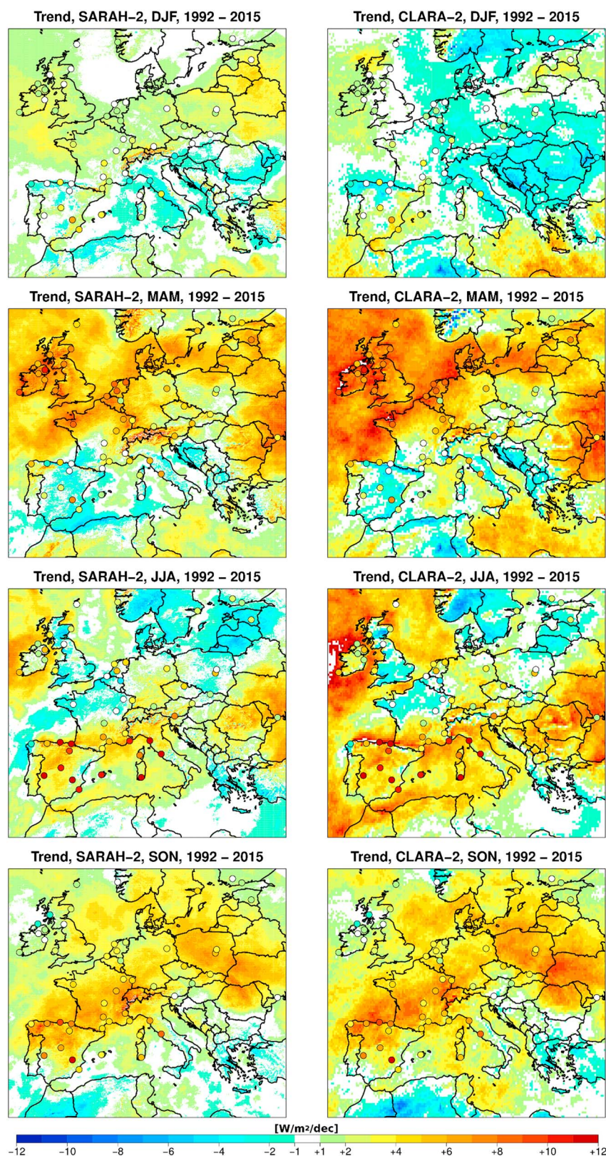
Figure 11. Spatial distribution of the linear trends ( \text{W/m}^2/\text{decade} ) of surface solar radiation during 1992–2015 for the four seasons (DJF, MAM, JJA, and SON) (top to bottom) based on the (left column) SARAH-2 and (right column) CLARA-A2 climate data records. The trends for the respective season and time period given by the stations are shown as colored dots.
