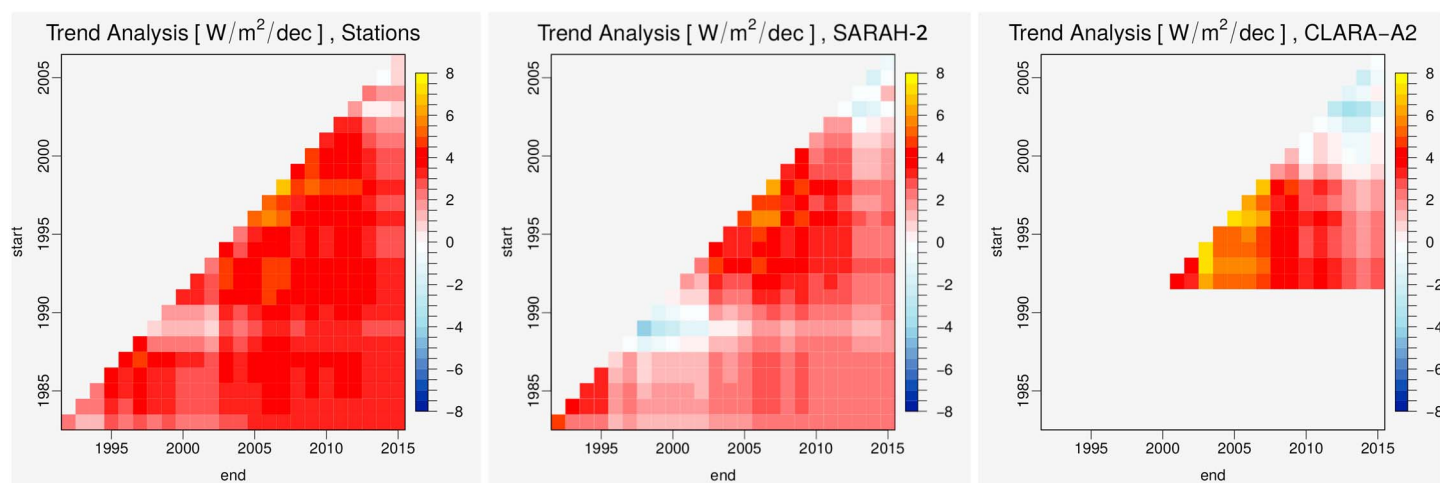
Figure 5. Trendraster-plots of mean SSR trends derived from (left) stations, (middle) SARAH-2, and (right) CLARA-A2. The y axis denotes the start years, and the x axis shows the end years of the individual trends. Trendrasters show linear trends ( \text{W/m}^2/\text{decade} ) during time periods of at least 10 years (at the diagonal); the trend over the maximum time period analyzed (33 years for station data and SARAH-2 and 24 years for CLARA-A2) is shown by the pixel at the lower right end.
