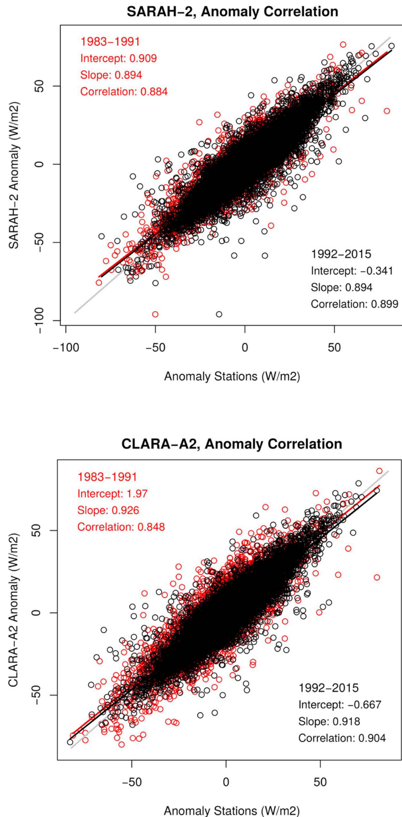
Figure 3. Scatterplot of monthly anomalies of surface solar radiation ( \text{W/m}^2 ) of (top) SARAH-2 and (bottom) CLARA-A2 versus station data, including correlation coefficient, slope, and intercept of the regression line. The red color refers to the 1983–1991 period, while the black color refers to the 1992–2015 period.
