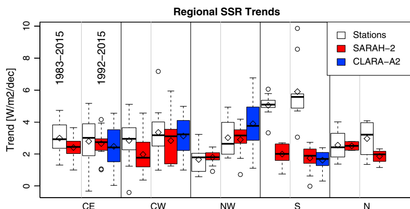
Figure 6. Box plot of the regional trends ( \text{W/m}^2/\text{decade} ) of surface solar radiation at the station locations (white) based on stations, (red) SARAH-2, and (blue) CLARA-A2 data, including mean trends (diamonds). Outliers are shown as dots. Regions: CE = central east, CW = central west, NW = northwest, S = south, and N = north. For each region the plot area is divided into trends for the full time period 1983–2015 (for stations and SARAH-2) and trends for the time period 1992–2015 (for stations, SARAH-2, and CLARA-A2).
