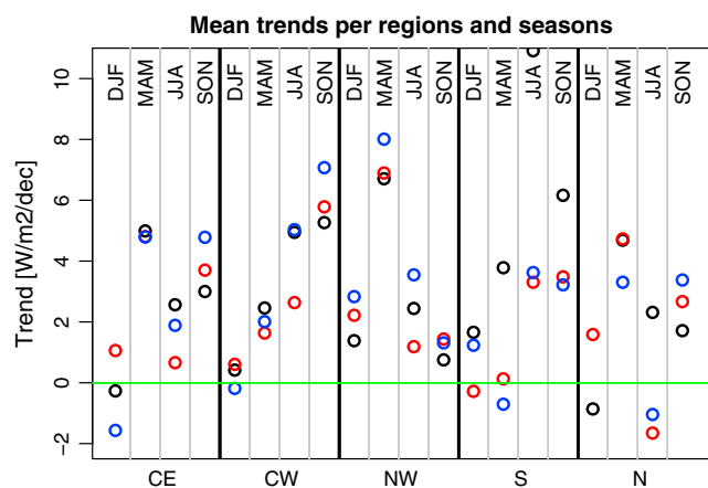
Figure 9. Trends ( \text{W/m}^2/\text{dec} ) of surface solar radiation of (black) stations, (red) SARAH-2, and (blue) CLARA-A2 data, shown separately for region and season during the time period of 1992–2015. Regions: CE = central east, CW = central west, NW = northwest, S = south, and N = north.
